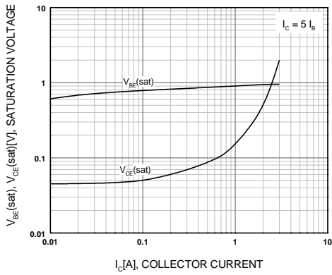
Figure 3. Collector-Emitter Saturation Voltage vs. Base-Emitter Saturation Voltage
